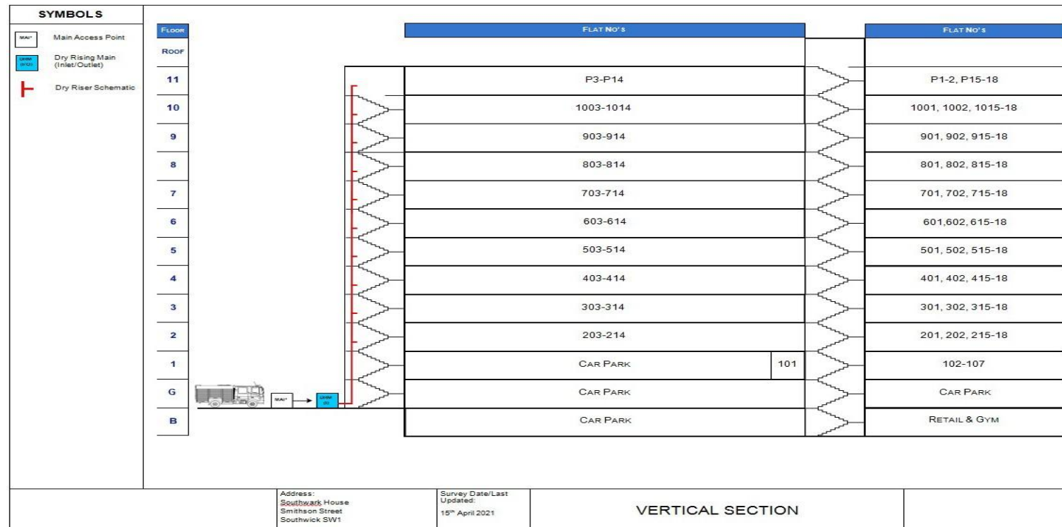
Figure 4: Example schematic showing fire and rescue service access level, floor numbers and flat numbers
