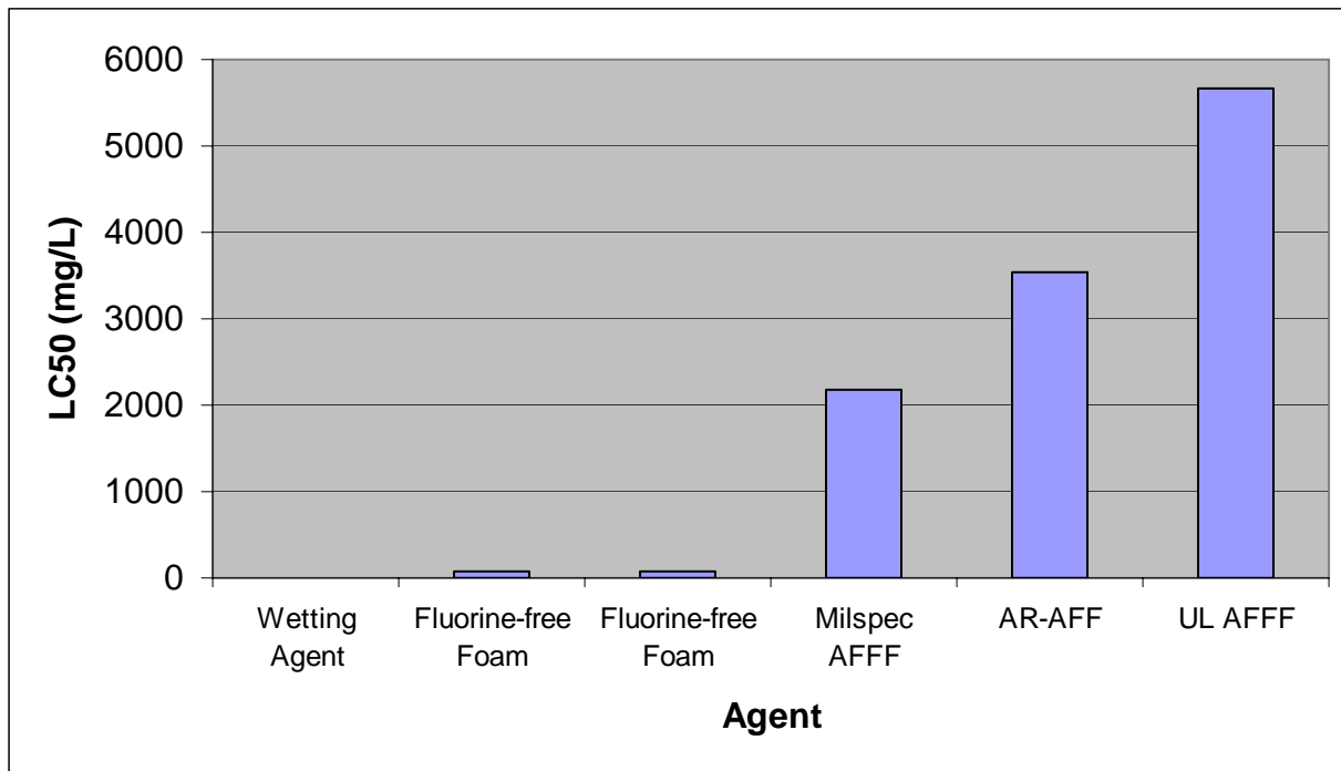
Figure 1 96-hour LC50 Test in Fingerling Rainbow Trout
