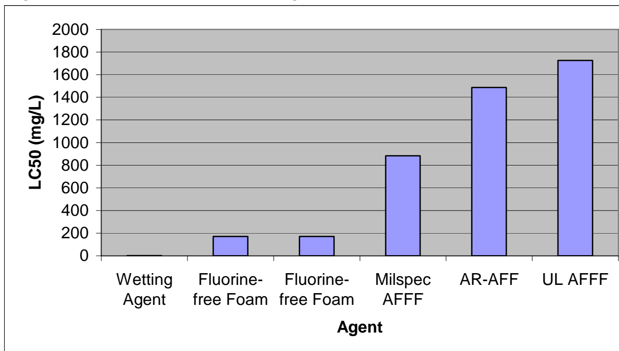
Figure 2 96-hour LC50 Flow-Through Test in Fathead Minnows
